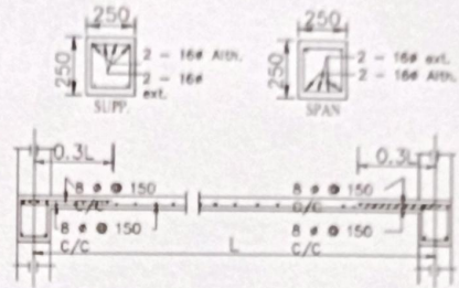
Details Of R.C.C Roof Slab & Beam (SCALE - 1 : 25)
