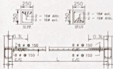
Details Of R.C.C Roof Slab & Beam
