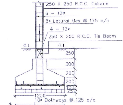
DETAILS OF R. C. C COLUMN (SCALE - 1 : 25)
