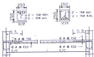
Details Of R.C.C Roof Slab & Beam (SCALE - 1 : 25)
