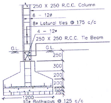
DETAILS OF R.C.C COLUMN (SCALE - 1 : 25)
