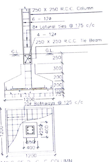
DETAILS OF R. C. C COLUMN (SCALE 1 : 25)
