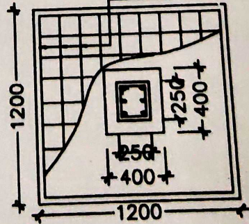
DETAILS OF R. C. C COLUMN (SCALE - 1 : 25)
