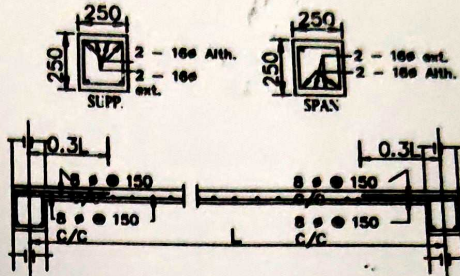
Details Of R.C.C Roof Slab & Beam
