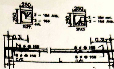
Details Of R.C.C Roof Slab & Beam (SCALE - 1 : 25)
