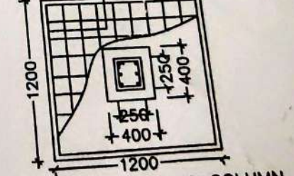
DETAILS OF R. C. C COLUMN (SCALE - 1 : 25)
