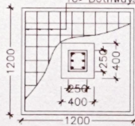
DETAILS OF R. C. C COLUMN
