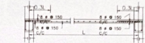
Details Of R.C.C Roof Slab & Beam
