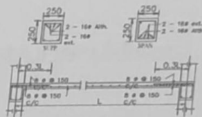
Details Of R.C.C Roof Slab & Beam (SCALE - 1 : 25)
