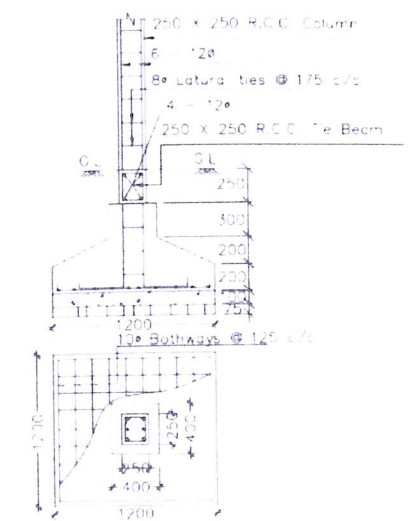
DETAILS OF R.C.C. COLUMN (SCALE - 1:25)
