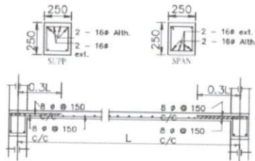
Details Of R.C.C Roof Slab & Beam (SCALE - 1 : 25)
